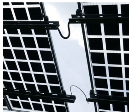
Simple electrical connection of the module tables
